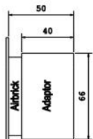
Airbrick 50 mm male connection to adaptor allowing + 40mm extension
